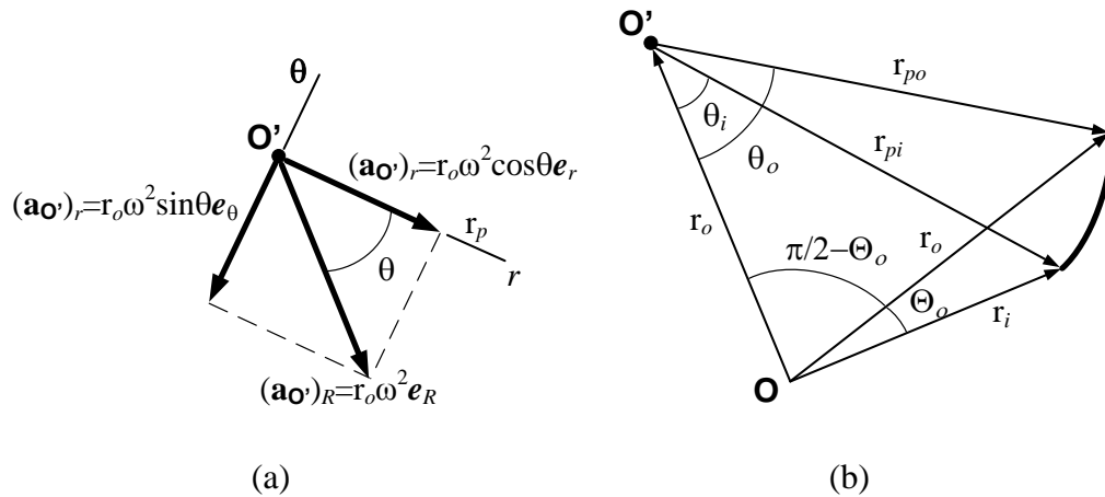
Figure 41. Transposition to the rotating coordinate system r - \theta ; (a) absolute radial acceleration of O' , and (b) radial position of leading and trailing edge of curved blade.
