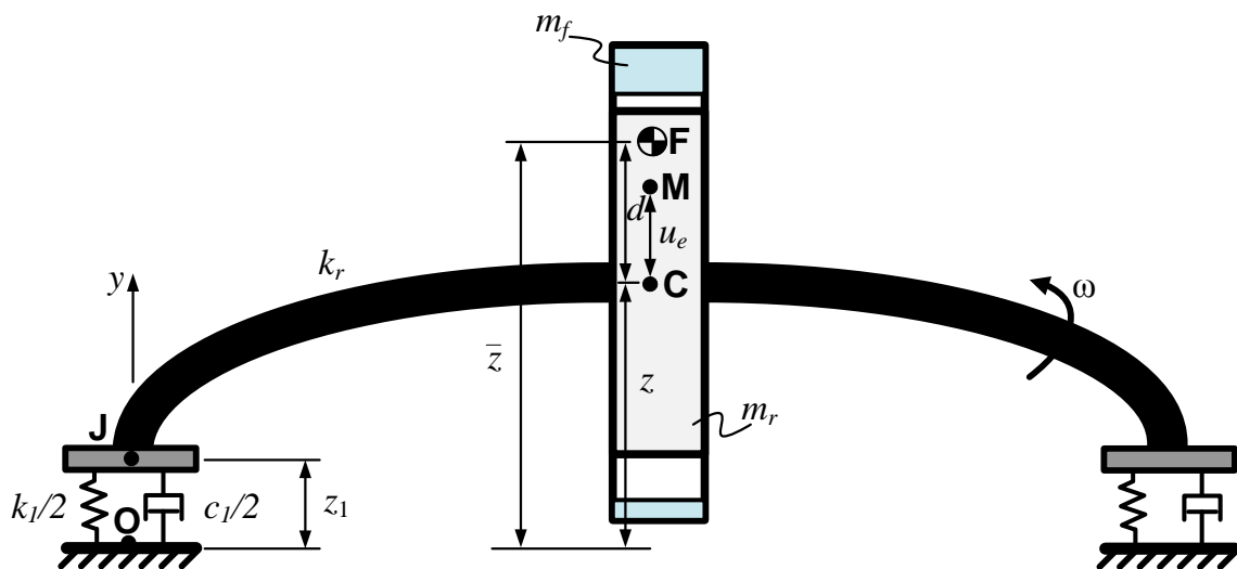
Figure 32. Dynamic model of a flexible rotor with a liquid balance ring.
